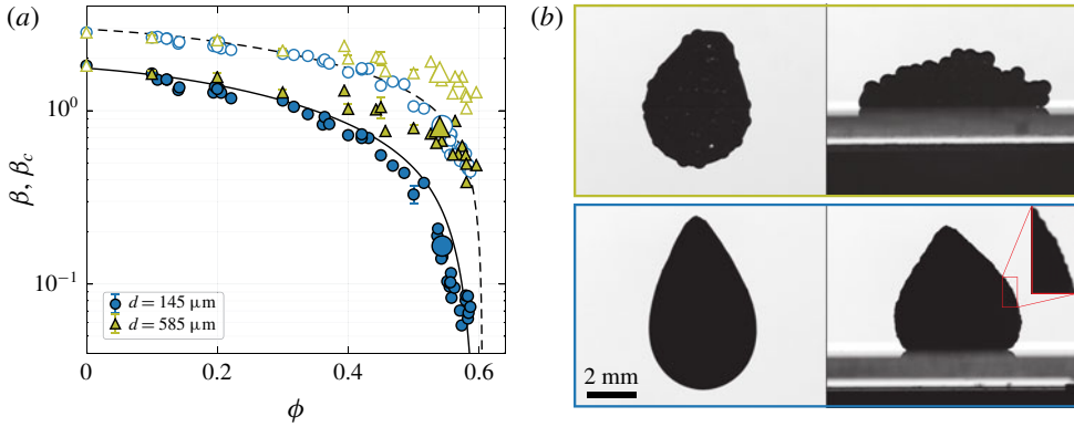
FIGURE 6. Influence of the particle size for the same suspending liquid and impact parameters ( \eta_0 = 50.5 mPa s, V = 4 m s ^{-1} ). (a) Spreading versus \phi (same data as in figure 2a for d = 145 \mu m). Filled (respectively, open) symbols correspond to \beta (respectively, \beta_c ). (b) Comparison of the drop deformations for the same volume fraction \phi = 0.54 (larger symbols in (a), the scale is the same for the two concentrations).
